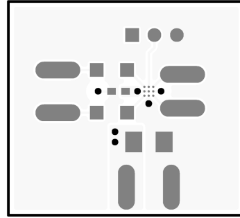
FIGURE 8. Top Layer
