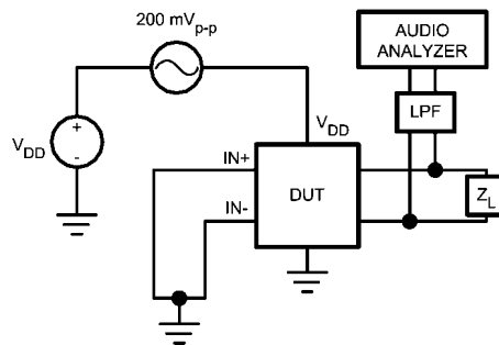
FIGURE 2. PSRR Test Circuit
