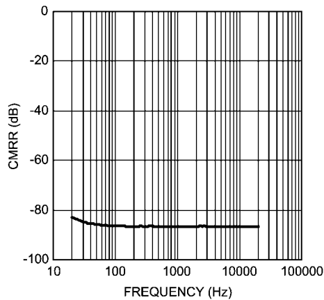
CMRR vs Frequency V_{DD} = 5.0\text{V}, V_{RIPPLE} = 1\text{V}_{P-P}, R_L = 8\Omega
