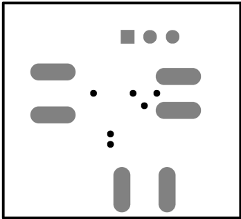
FIGURE 9. Bottom Silkscreen
