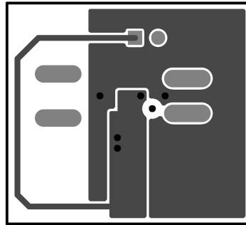
FIGURE 10. Bottom Layer
