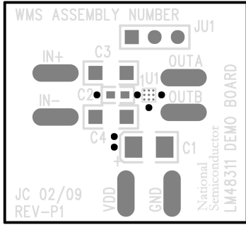
FIGURE 7. Top Silkscreen
