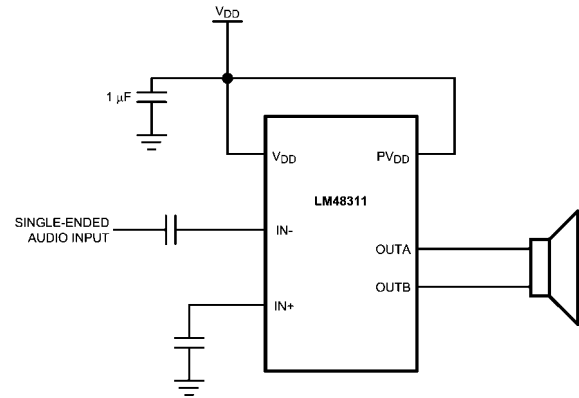
FIGURE 5. Single-Ended Input Configuration
