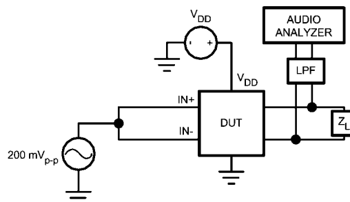
FIGURE 3. CMRR Test Circuit
