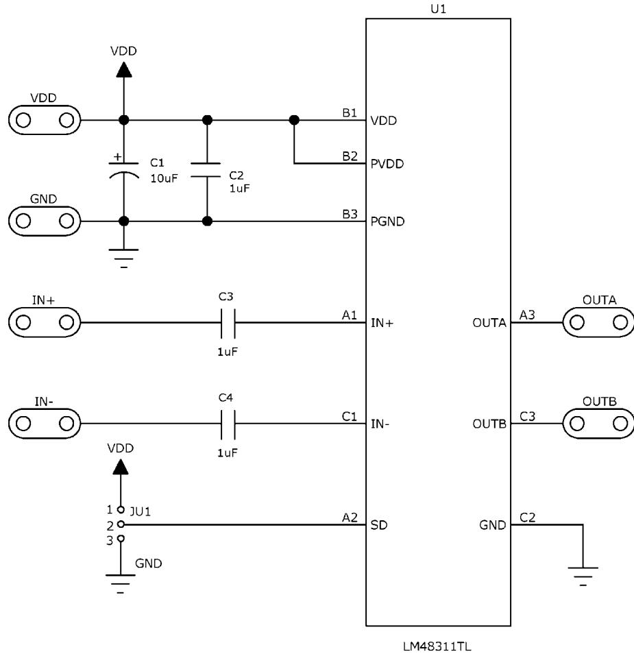
FIGURE 6. LM48311 DEMO BOARD SCHEMATIC
