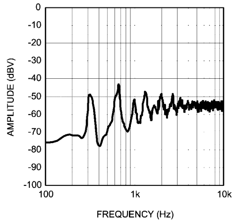
Wideband Spread Spectrum Output Spectrum vs Frequency V_{DD} = 5V, R_L = 8\Omega
