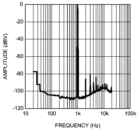
Spread Spectrum Output Spectrum vs Frequency V_{DD} = 5V, V_{IN} = 1V_{RMS}, R_L = 8\Omega
