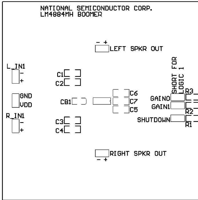
FIGURE 2. Recommended MH PC Board Layout: Component-Side Silkscreen
