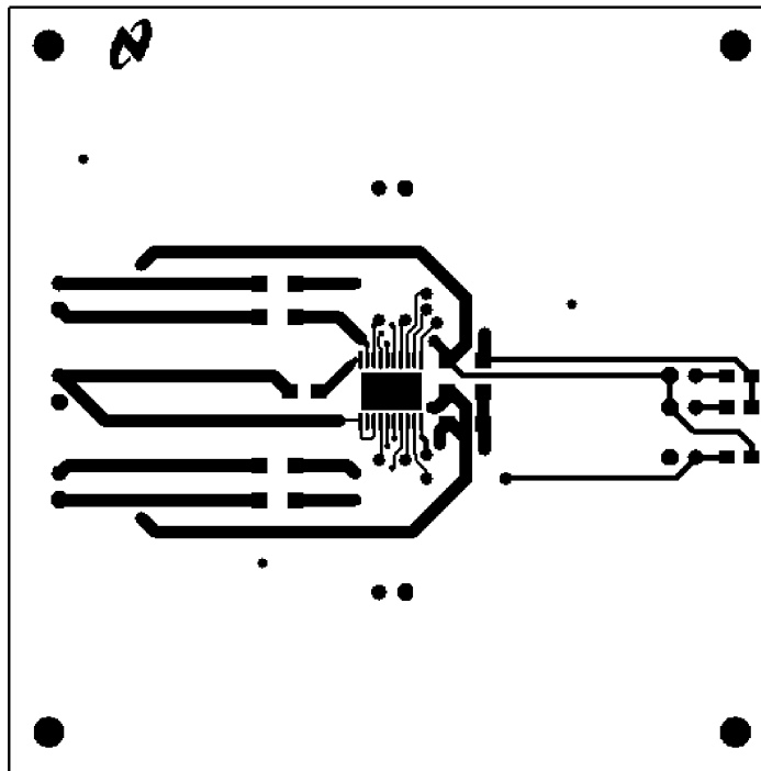
FIGURE 3. Recommended MH PC Board Layout: Component-Side Layout
