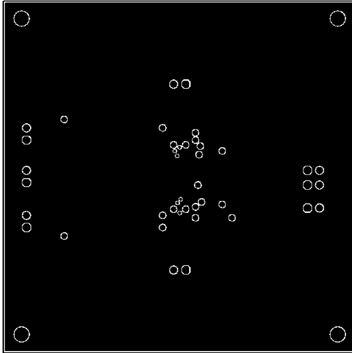
FIGURE 6. Recommended MH PC Board Layout: Bottom-Side Layout
