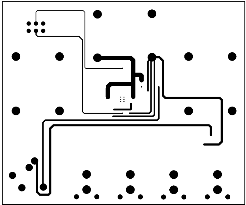
FIGURE 6. Bottom Layer
