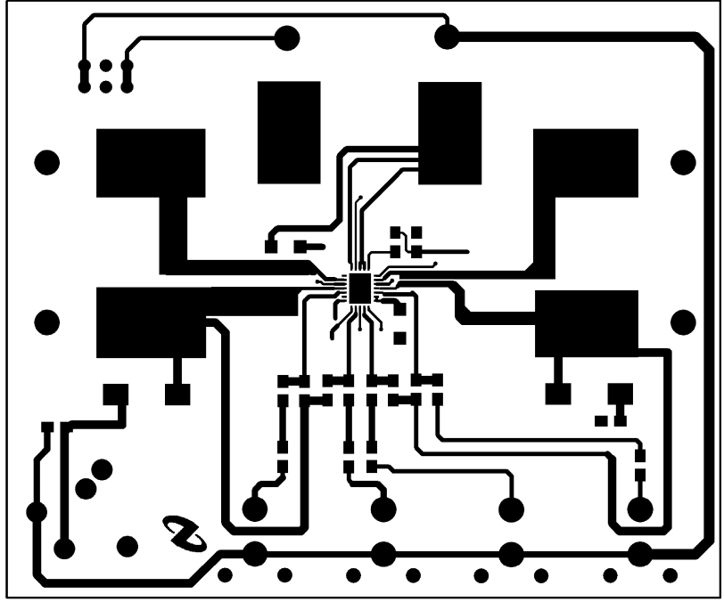
FIGURE 5. Top Layer
