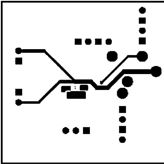
FIGURE 9: Bottom Layer
