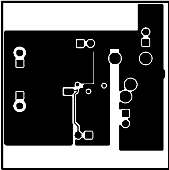
FIGURE 7: Layer 2
