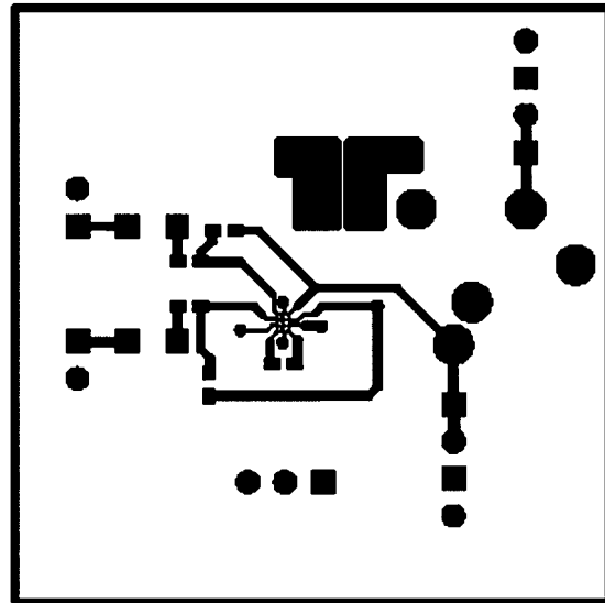
FIGURE 6: Top Layer 30054109
