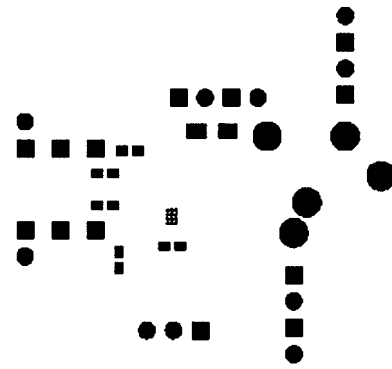
FIGURE 4: Top Solder Mask 30054199
