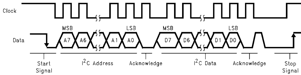
FIGURE 3. I 2 C Bus Format
