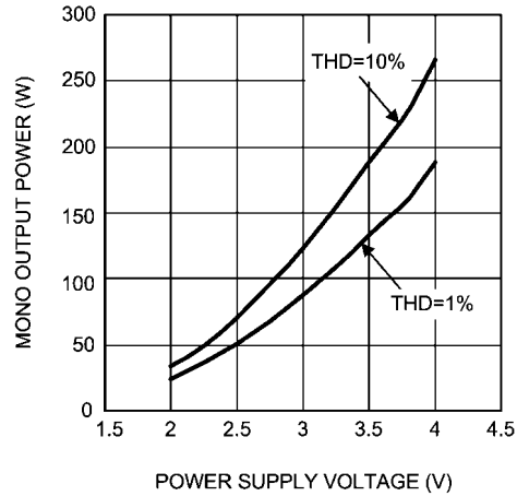
Output Power vs Voltage Supply R_L = 16\Omega, \text{Mono}
