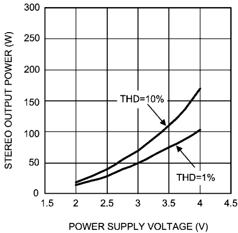
Output Power vs Voltage Supply R_L = 32\Omega, \text{Stereo}
