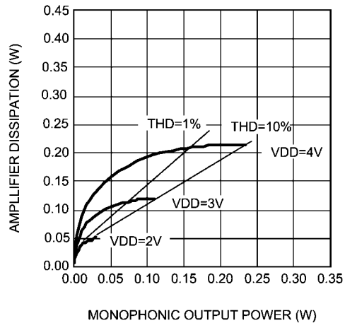
Output Power vs Power Dissipation V_{DD} = 2V, 3V, 4V, R_L = 16\Omega, \text{Mono}
