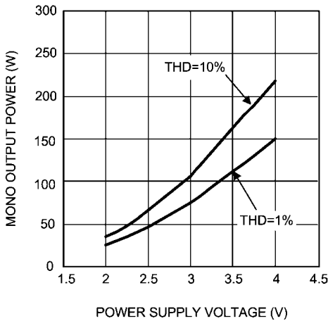
Output Power vs Voltage Supply R_L = 32\Omega, \text{Mono}
