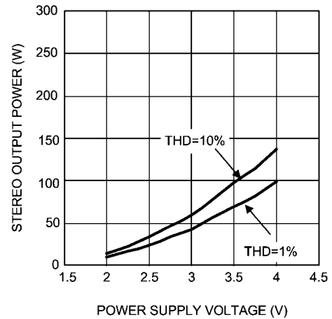
Output Power vs Voltage Supply R_L = 16\Omega, \text{Stereo}
