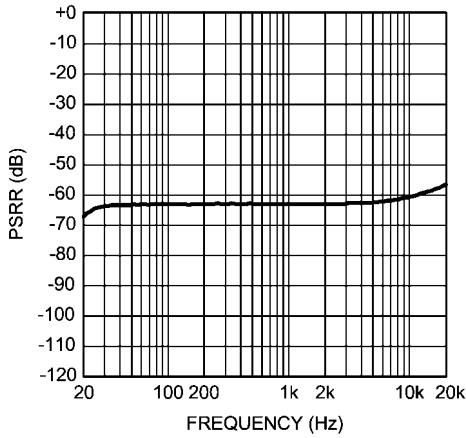
PSRR vs Frequency V_{DD} = 4V, R_L = 32\Omega
