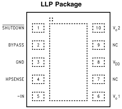
Top View Order Number LM4892LD See NS Package Number LDA10B
