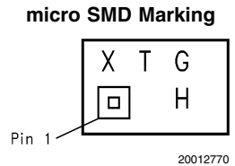
Top View X - Date Code T - Die Traceability G - Boomer Family H - LM4892IBP
