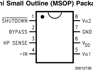
Top View Order Number LM4892MM See NS Package Number MUA08A
