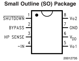
Top View Order Number LM4892M See NS Package Number M08A
