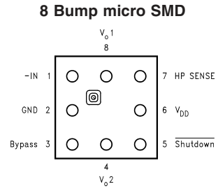
Top View Order Number LM4892IBP, LM4892IBPX See NS Package Number BPA08DDB
