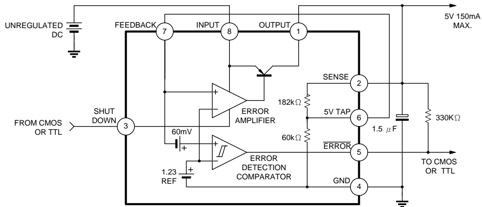
FOR UTC LP2951
