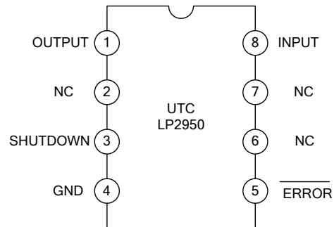
SOP-8 OR DIP-8 PACKAGE FOR UTC LP2950
