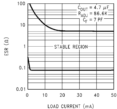
4.7 \mu F ESR Curves
