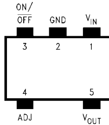
Top View See NS Package Number MF05A
