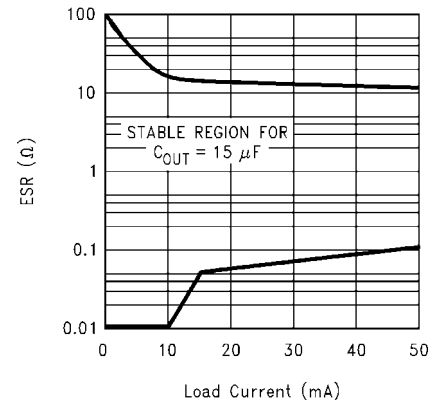
15 \mu\text{F} ESR Curves For 1.8V Output 10109121
