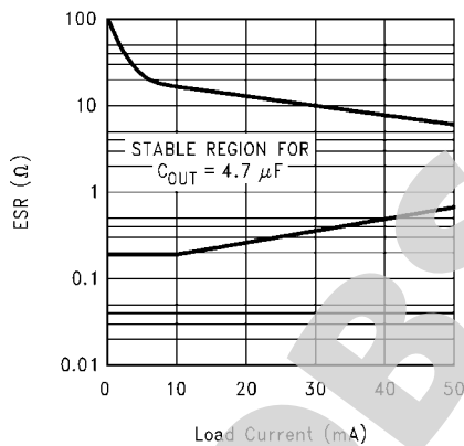
4.7 \mu\text{F} ESR Curves For 1.8V Output 10109119
