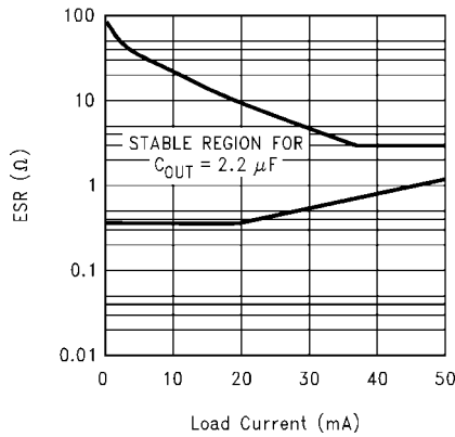
2.2 \mu\text{F} ESR Curves For 1.8V Output 10109118
