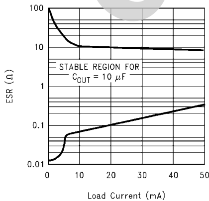
10 \mu\text{F} ESR Curves For 1.8V Output 10109120
