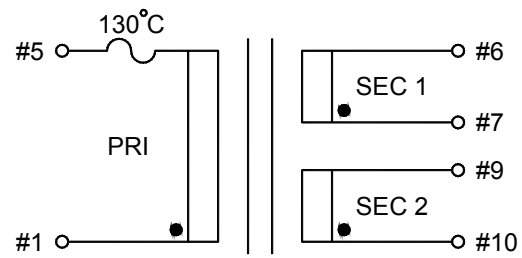
Double Output
