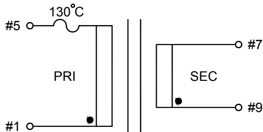
Single Output
