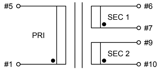
Double Output
