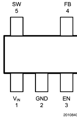
FIGURE 3. Top View SOT23-5 Package NS Package Number MF05A (2.92mm x 2.84mm x 1.2mm)
