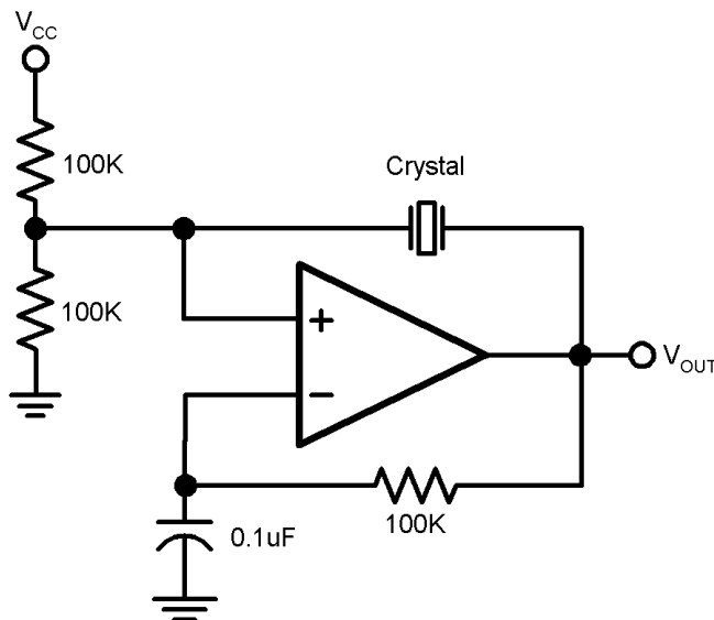
Crystal Oscillator
