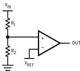
FIGURE 4. Threshold Detector
