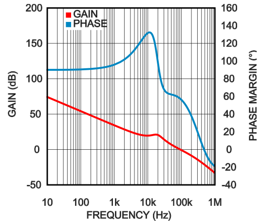
FIGURE 11. Loop Response
