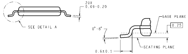
DETAIL A TYPICAL
