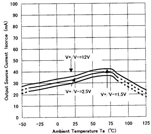
NJM13404 Output Source Current vs. Temperature
