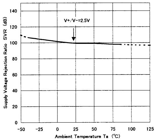
NJM13404 Supply Voltage Rejection Ratio vs. Temperature
