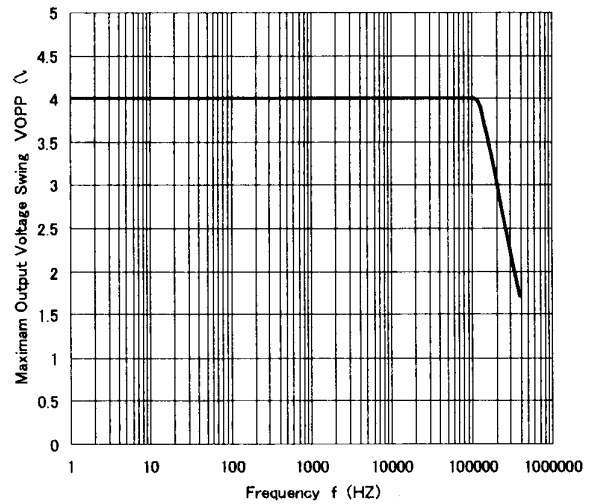
NJM13404 Maximum Output Voltage Swing v.s Frequency
