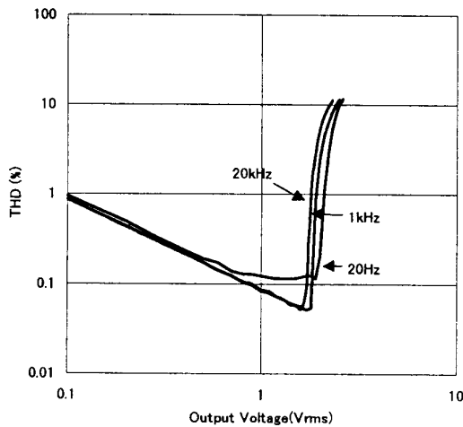
NJM13404 THD v.s Output Voltage
