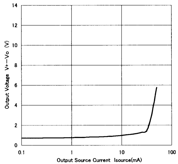
NJM13404 Output Voltage v.s Output Source Current
