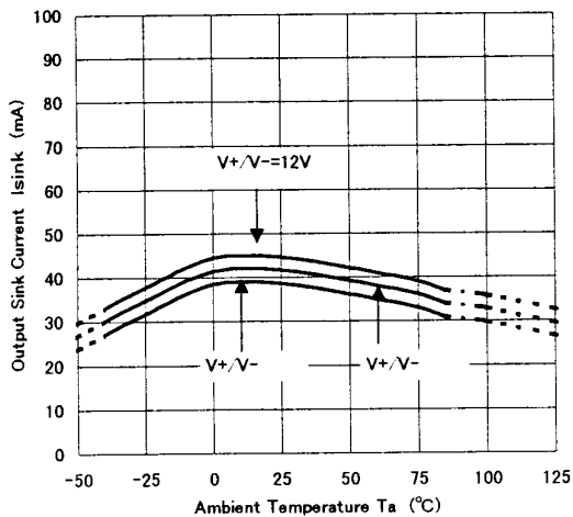
NJM13404 Output Sink Current vs. Temperature
