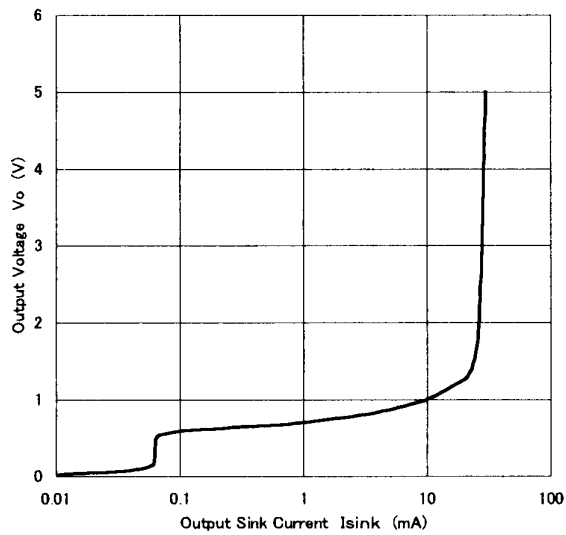
NJM13404 Output Voltage v.s Output Sink Current
