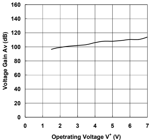
Voltage Gain vs. Operating Voltage (Ta=25°C, R L =2kΩ)
