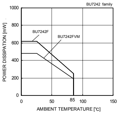
Fig. 1 Derating curve
