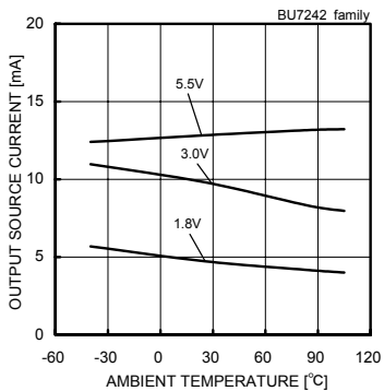
Fig. 10 Output Source Current - Ambient Temperature (VOUT=VDD-0.4[V])
