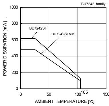
Fig. 2 Derating curve
