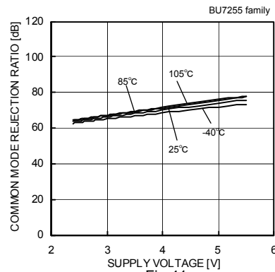
Fig.41 Common Mode Rejection Ratio – Supply Voltage (VDD=3[V])
