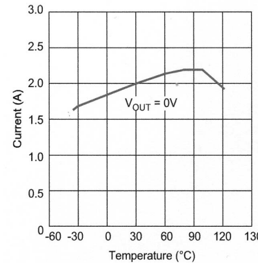
Figure 8. LM29150-3.3 Short Circuit Current vs. Temperature
