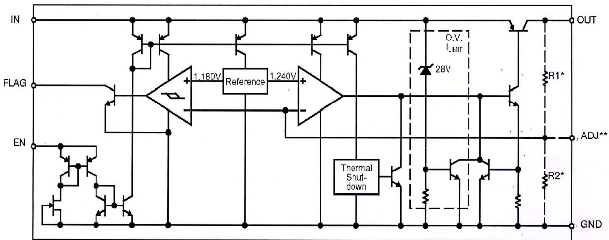
[ Block Diagram ]
