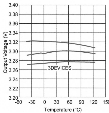
Figure 7. LM29150-3.3 Output Voltage vs. Temperature
