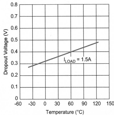
Figure 2. LM29150 Dropout Voltage vs. Temperature
