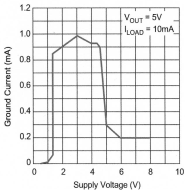
Figure 4. LM29150 Ground Current vs. Supply Voltage
