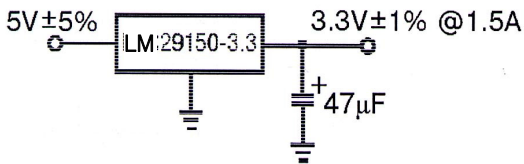
Figure1. Fixed output voltage
