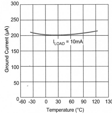
Figure 5. LM29150 Ground Current vs. Temperature
