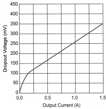
Figure 1. LM29150 Dropout Voltage vs. Output Current
