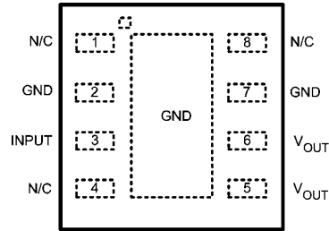
882246 Top View See NS Package Number LDC08A Pin 2 and pin 7 are fused to center DAP Pin 5 and 6 need to be tied together on PCB board
