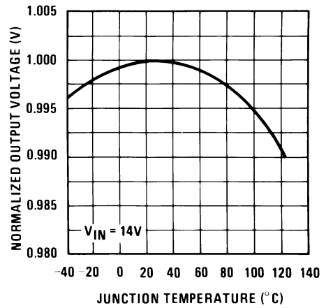
Output Voltage (Normalized to 1V at T_j=25^\circ\text{C} )
