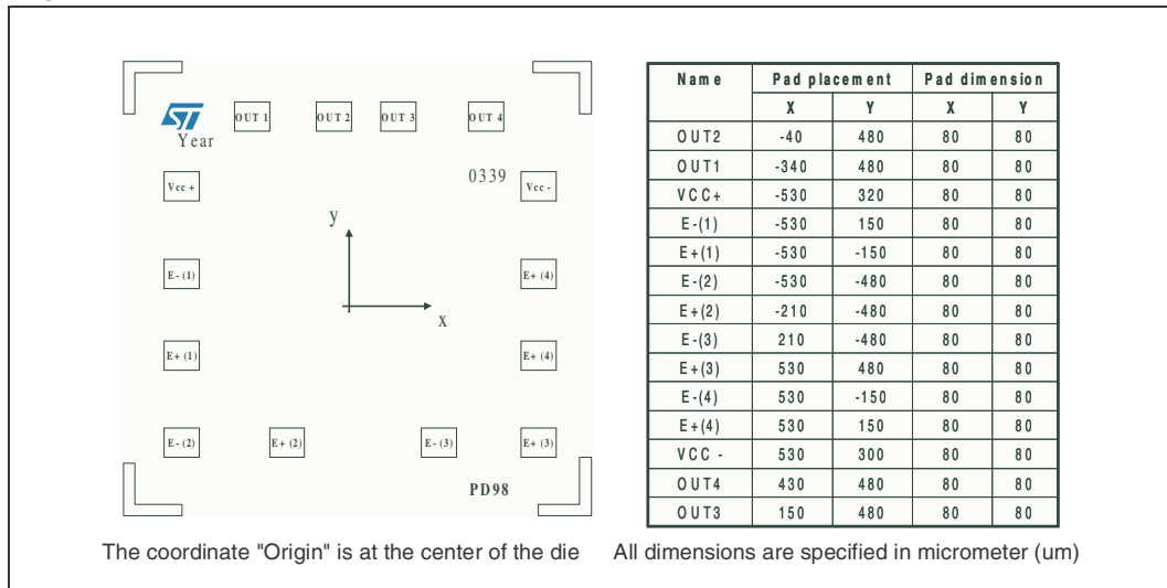
Figure 2. Pad locations
