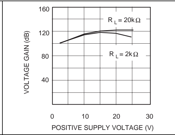
Figure 16. Voltage gain
