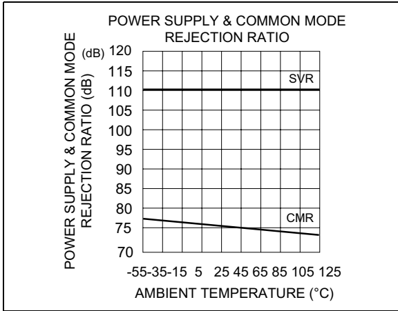
Figure 17. Power supply and common mode rejection ratio
