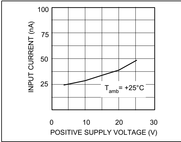
Figure 15. Input current
