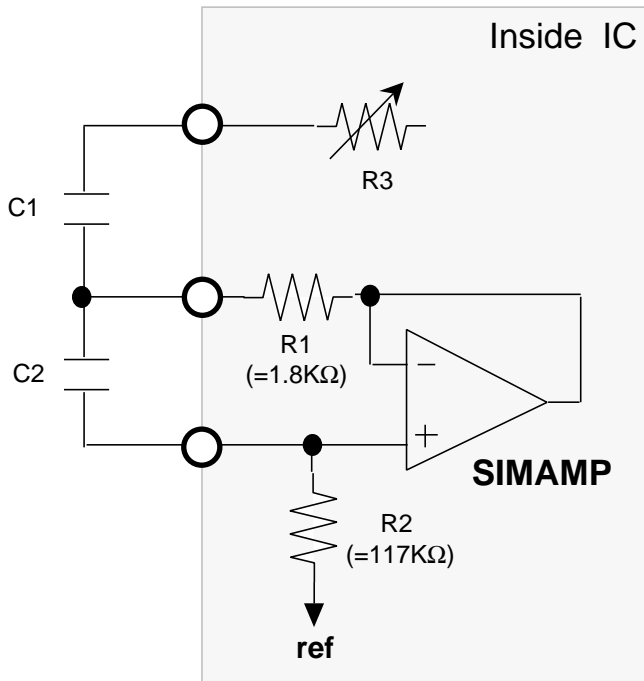
FIG1. The circuit used simulated inductor.
