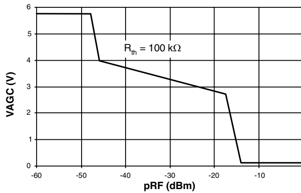
Figure 4. Gain Control Voltage (Pin 11)
