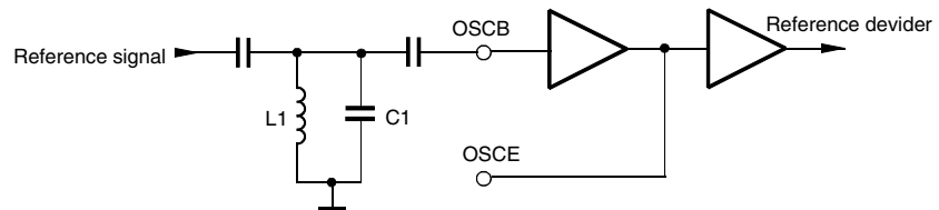
Figure 11. Reference Oscillator Overdriven
