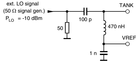
Figure 9. Application Circuit for External LO Signal
