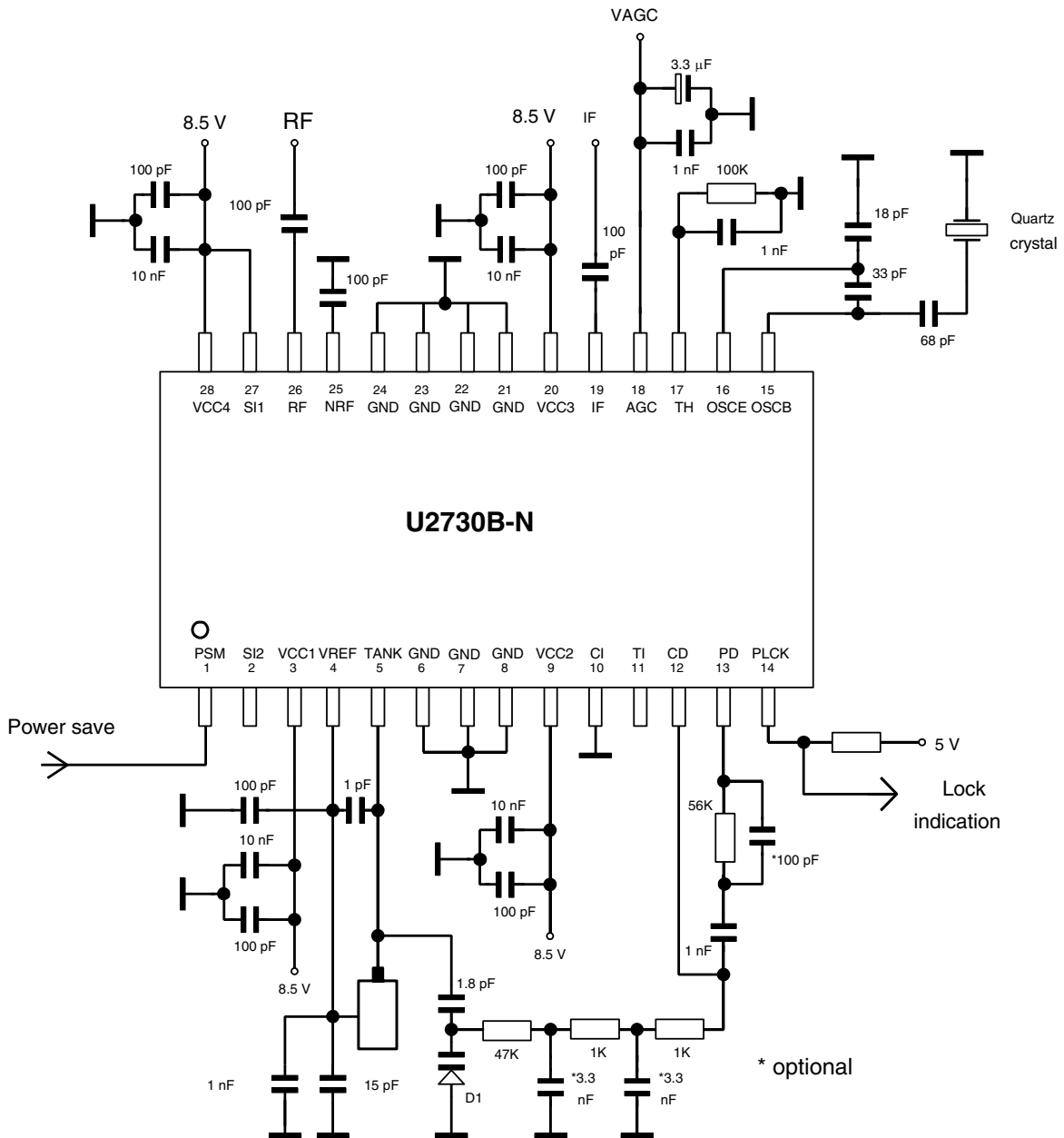
Figure 8. Application Circuit
