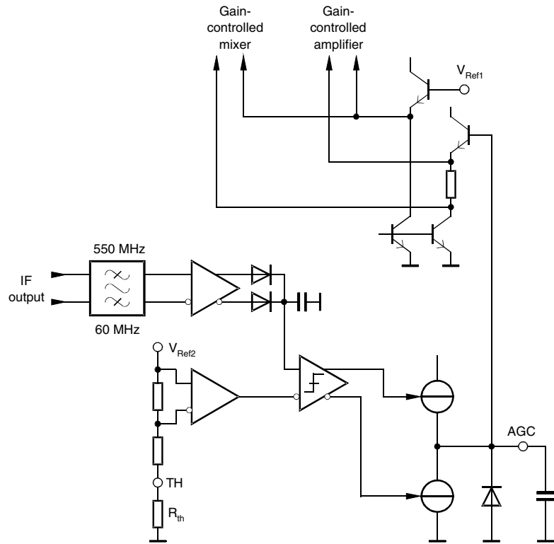
Figure 6. AGC Control Circuit
