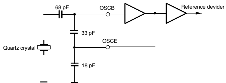
Figure 10. Reference Oscillator Operation
