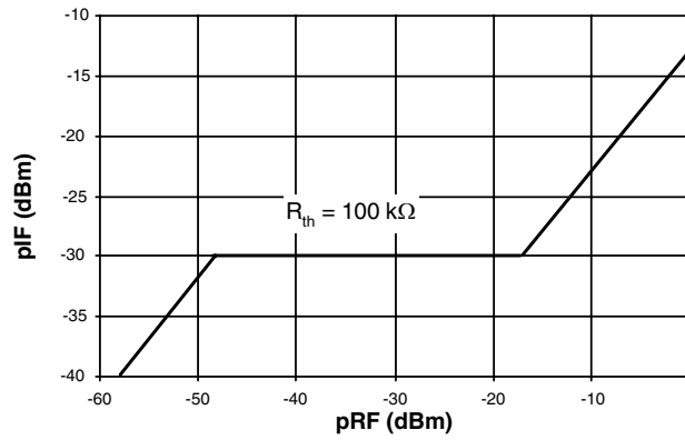
Figure 3. IF Output Power (Pin 19)
