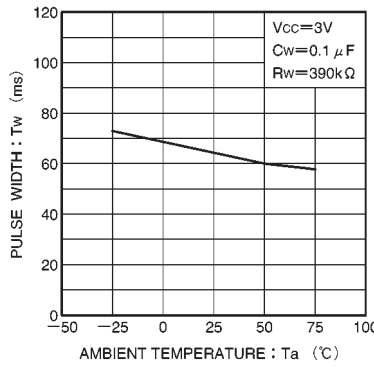
Fig. 15 Output pulse width vs. ambient temperature
