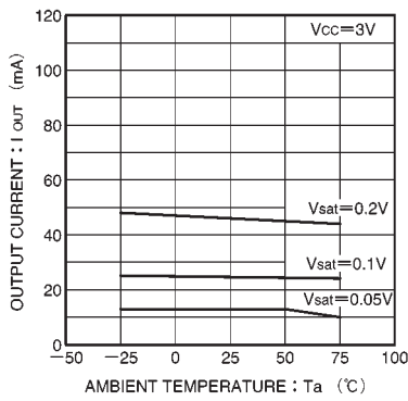
Fig. 23 Output current vs. ambient temperature
