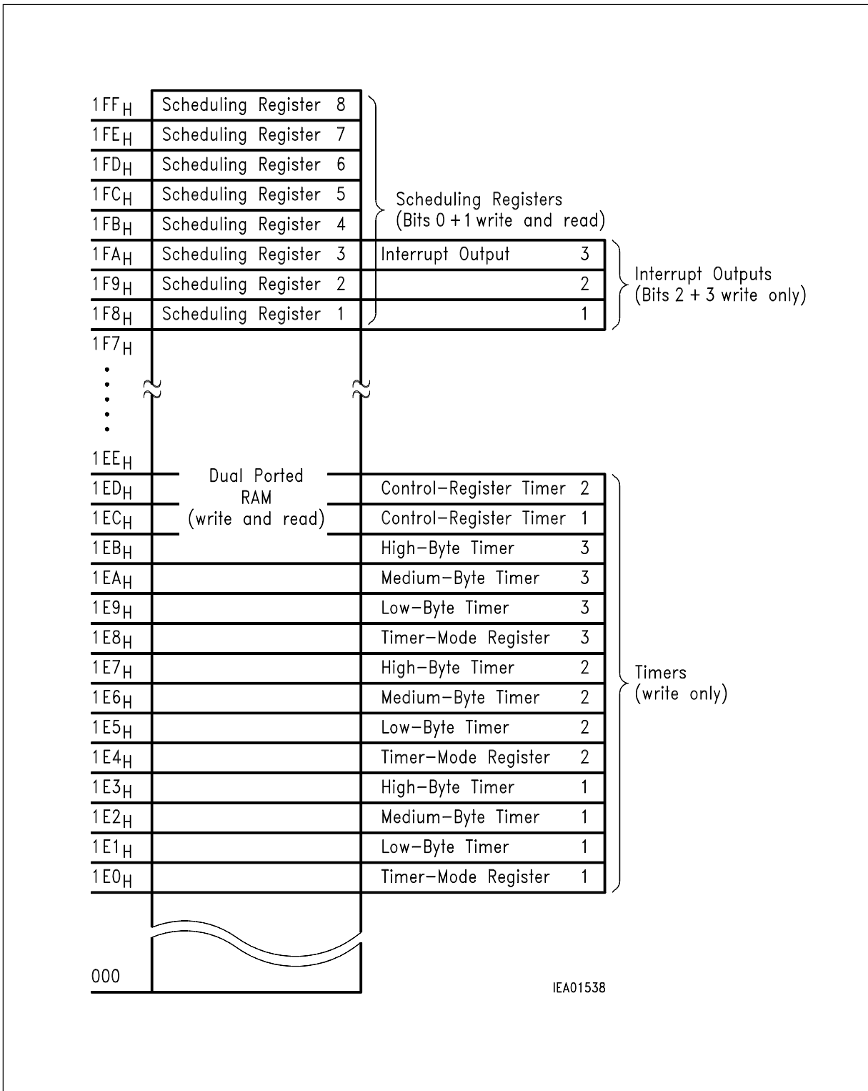
Figure 7 Memory Map
