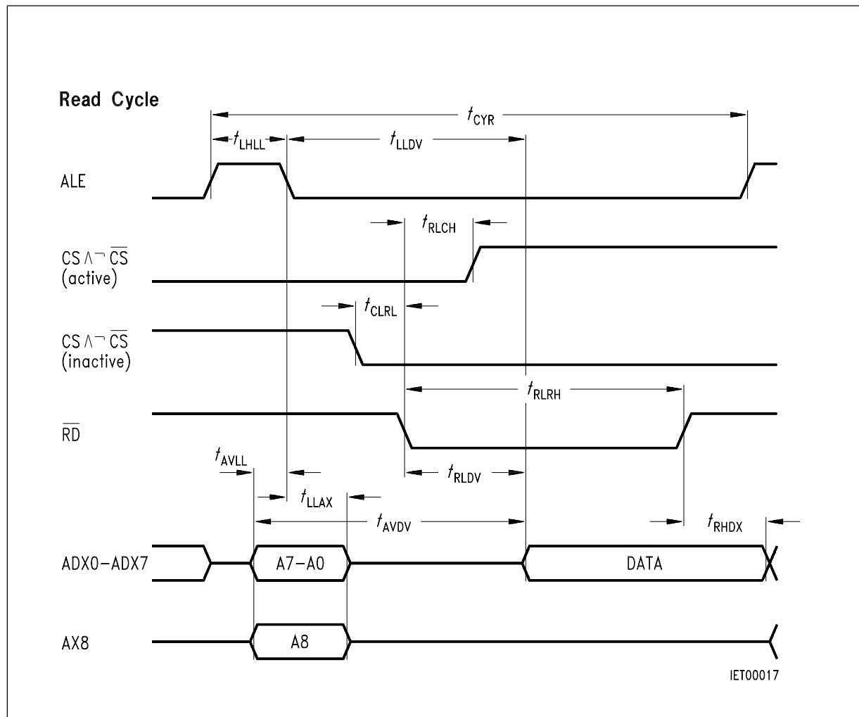
Pulse Diagram 1
