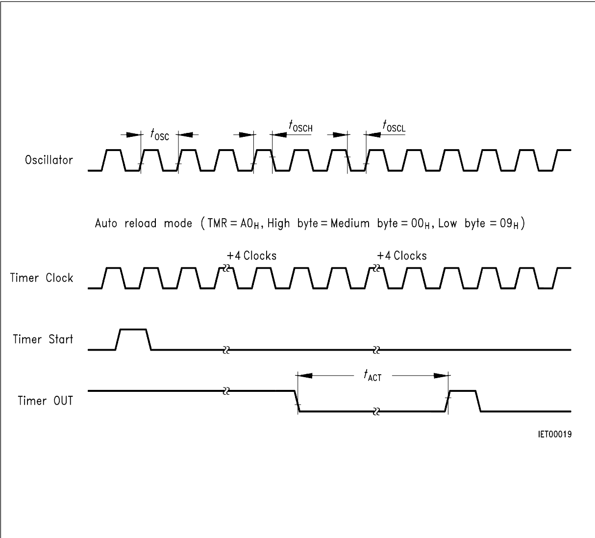
Pulse Diagram 3
