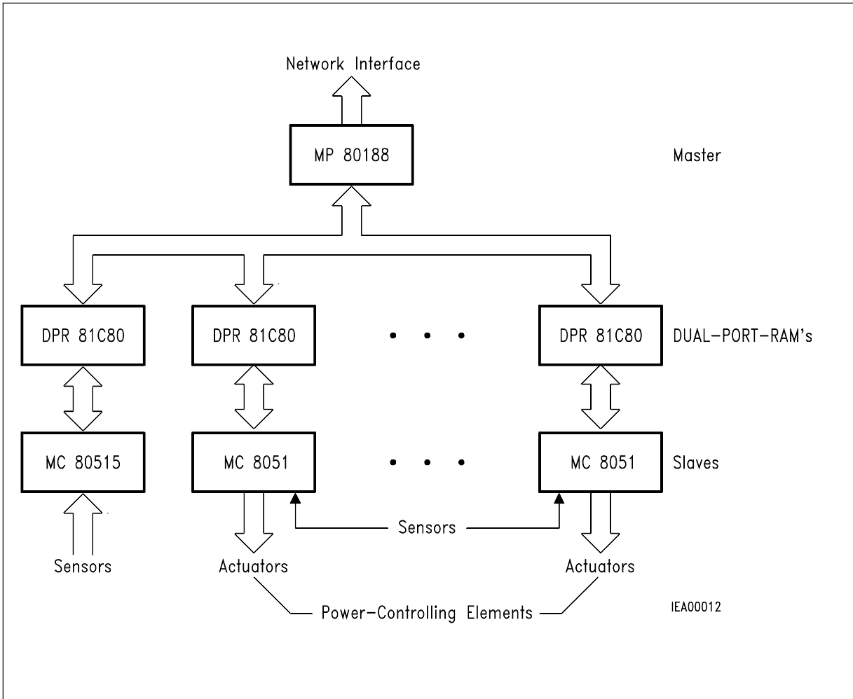
Figure 2 Interfacing Master and Slave Processors by DPRs
