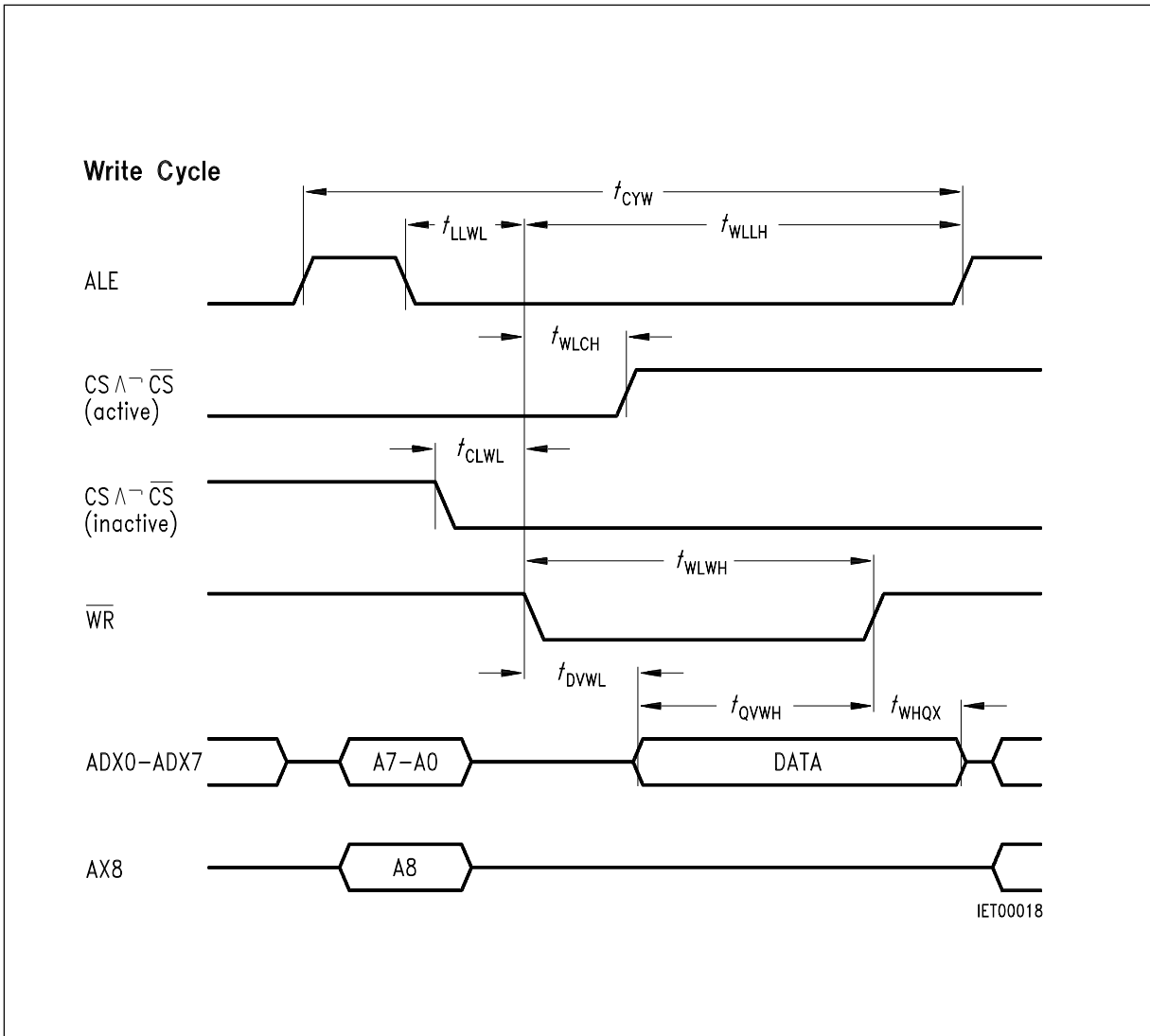
Pulse Diagram 2
