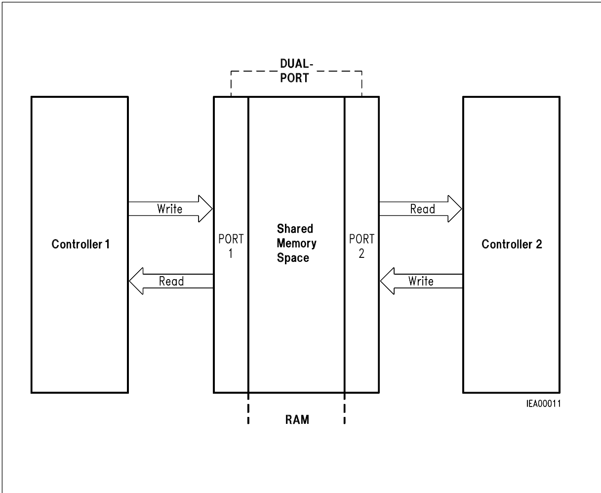
Figure 1 Principle of the Dual-Port-RAM (DPR)
