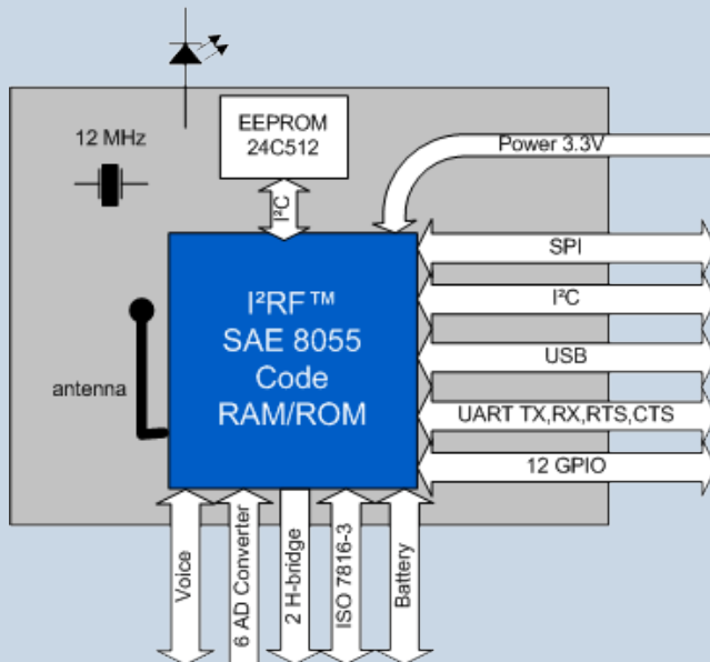
Application Block Diagram
