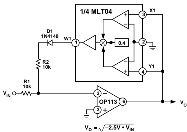
Voltage-Controlled Low-Pass Filter
