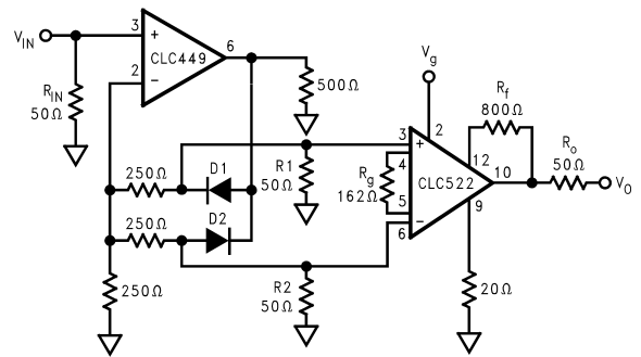
FIGURE 10. Full-Wave Rectifier
