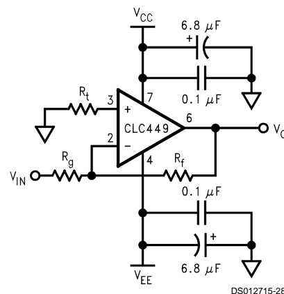
FIGURE 2. Inverting Gain
