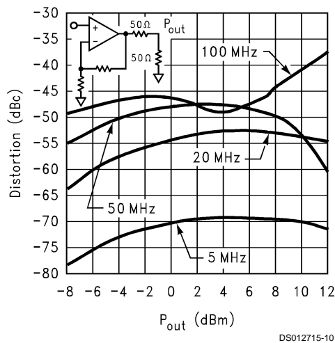
2nd Harmonic Distortion vs. P_{out}
