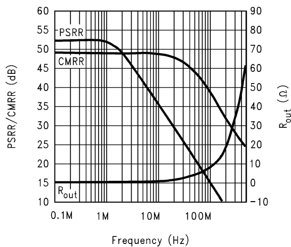
PSRR, CMRR, and Closed Loop R_{\text{OUT}}
