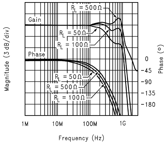
Frequency Response vs. Load
