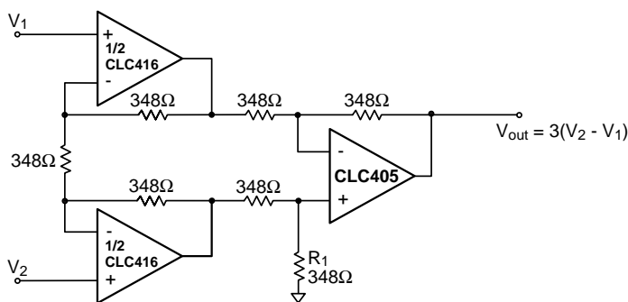
Typical Application Diagram Instrumentation Amplifier
