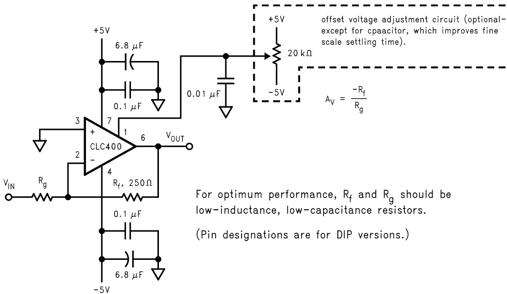
FIGURE 2. Recommended Inverting Gain Circuit
