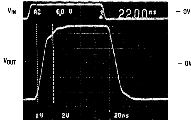
Large Signal Response
