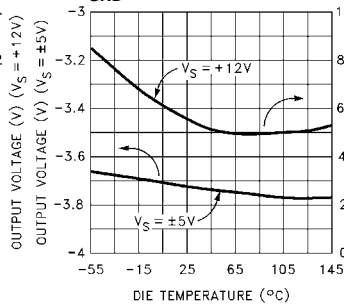
Negative Output Voltage Swing vs Die Temperature, R L = 150Ω to GND
