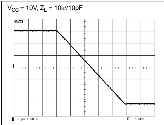
Figure 30. Large signal response - Amplifiers C to N
