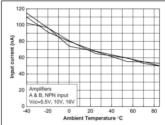
Figure 4. Input current ( I_{IB} ) vs. temperature
