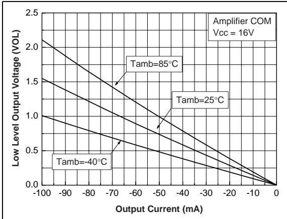
Figure 20. Voltage output low ( V_{OL} ) vs. output current - Amplifier COM
