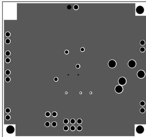
Recommended ITL PC Board Layout: Bottom Layer
