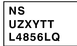
Top View NS - Std NS Logo U - Wafer Fab Code Z - Assembly Plant Code XY - 2 Digit Date Code TT - Die Run Traceability L4856LQ - LM4856LQ
