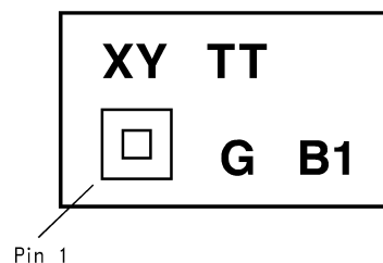
18-Bump micro SMD Marking (ITL)
