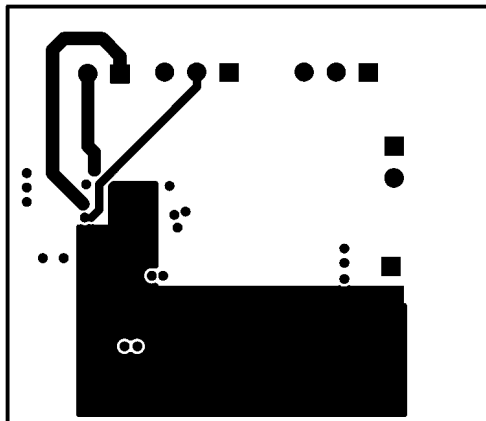
FIGURE 8. Bottom Layer
