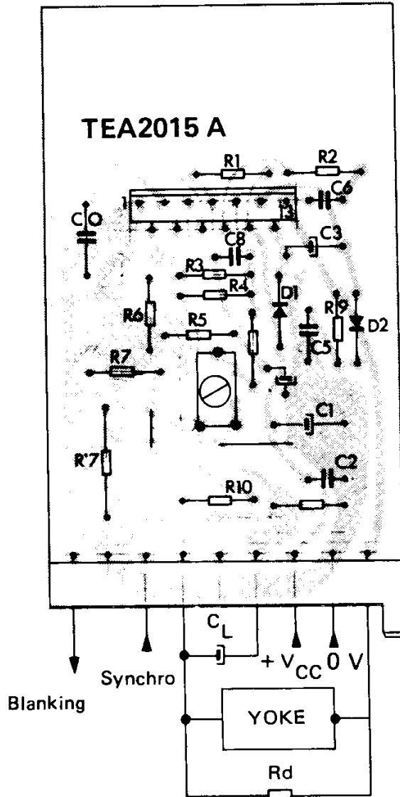
COMPONENT SIDE
