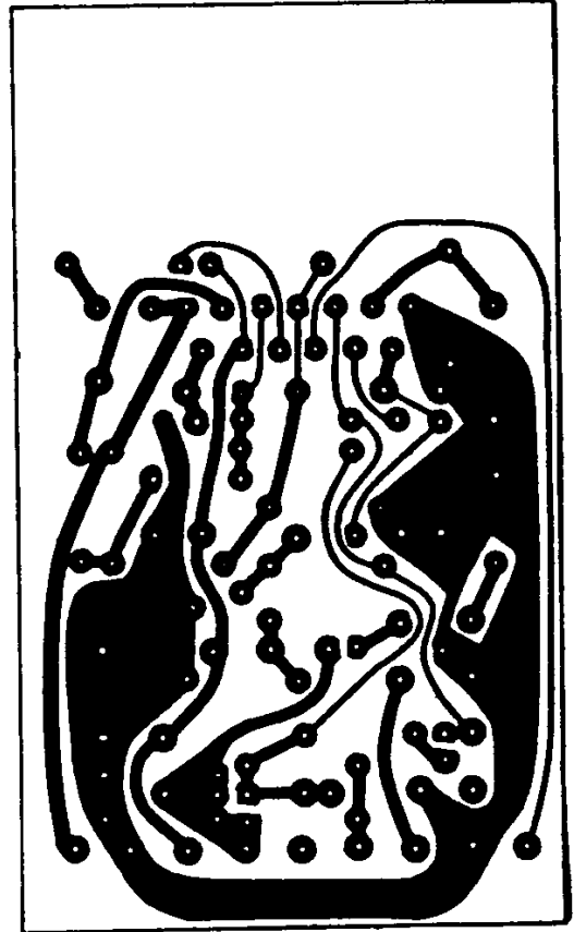
COPPER SIDE
