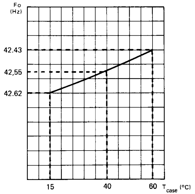
FREQUENCY VARIATION OF UNSYNCHRONIZED OSCILLATOR VERSUS TEMPERATURE
