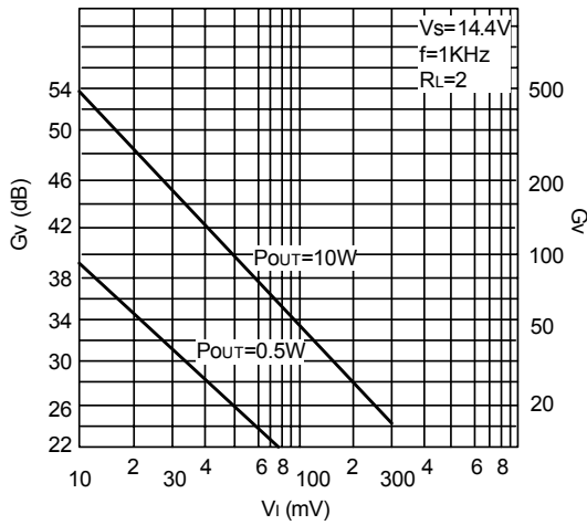
Figure 22. Gain versus Input Sensitivity (Stereo amplifier)
