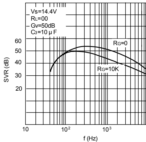
Figure 18. Supply Voltage Rejection versus Frequency (Stereo amplifier)
