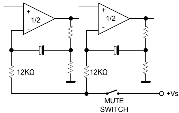
Figure 1. Example of Muting Circuit
