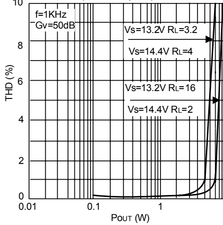
Figure 12. Distortion versus Output Power (Stereo amplifier)
