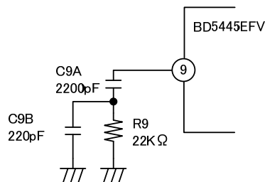
Fig.32 ROSC terminal filter circuit for setting slave mode.
