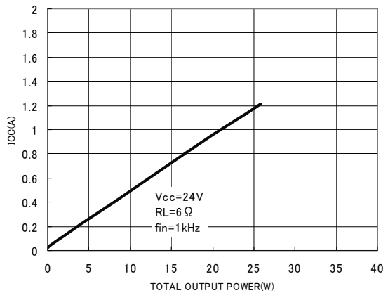
Fig.18 Total output power—Current consumption (RL=6Ω)
