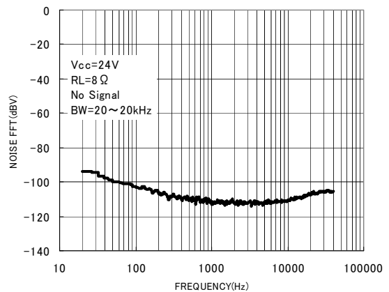
Fig.8 FFT of Output Noise Voltage
