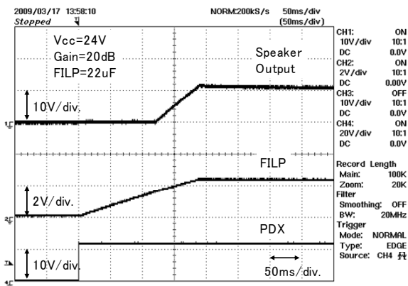
Fig.9 Waveform when releasing Power-down
