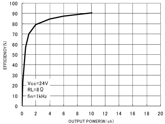
Fig.14 Output power—Efficiency (RL=8Ω)
