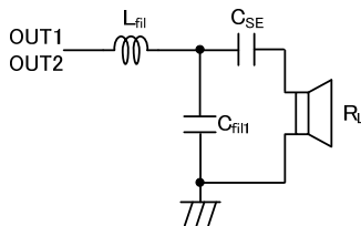
Fig.30 SE filter configuration
