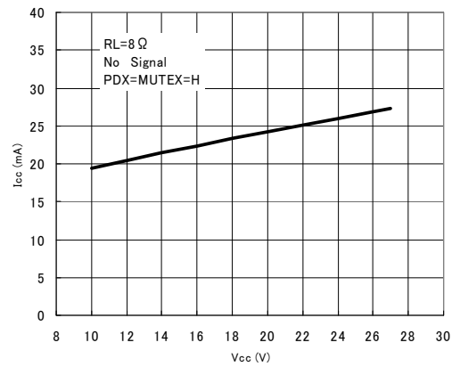
Fig. 2 Power supply voltage—Current consumption
