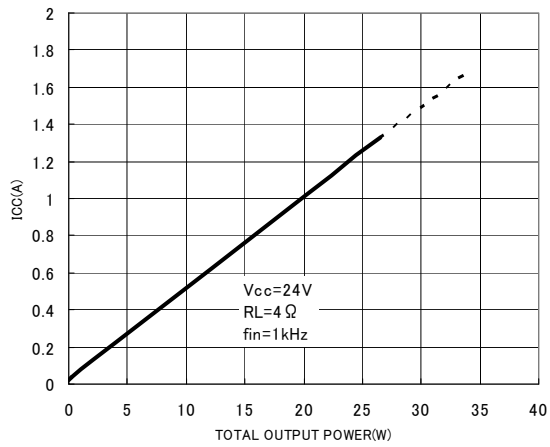
Fig.21 Total output power—Current consumption (RL=4Ω)
