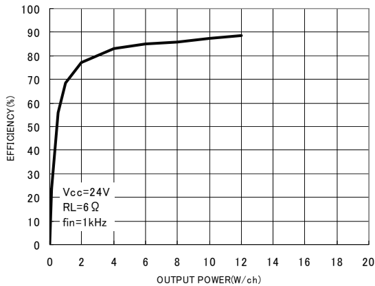
Fig.17 Output power—Efficiency (RL=6Ω)
