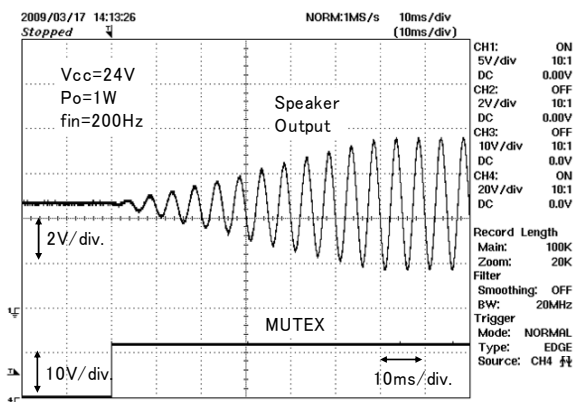
Fig.11 Waveform when releasing Soft-mute
