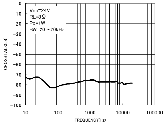
Fig.6 Frequency—Crosstalk
