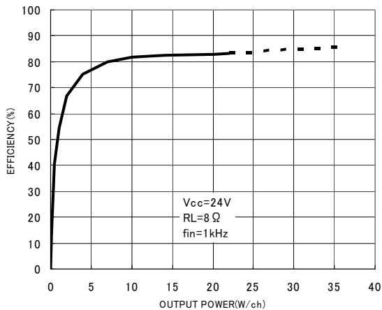
Fig.27 Output power—Efficiency ( R_L=8\Omega )
