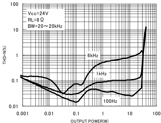
Fig.22 Output power—THD+n
