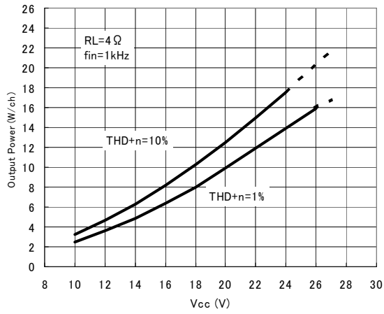
Fig.19 Power supply voltage—Output power (RL=4Ω)
