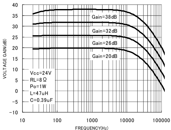
Fig.24 Frequency—Voltage gain
