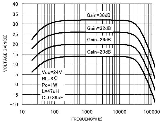
Fig.7 Frequency—Voltage gain
