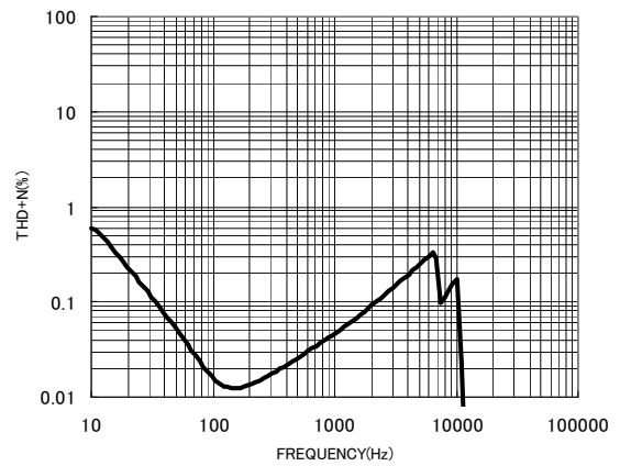
Fig.4 Frequency—THD+N
