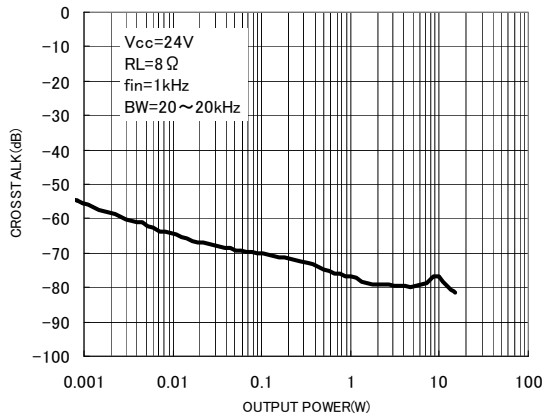
Fig.5 Output power—Crosstalk
