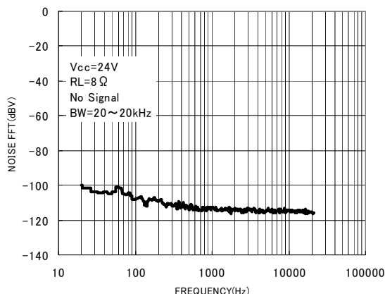
Fig.25 FFT of Output Noise Voltage
