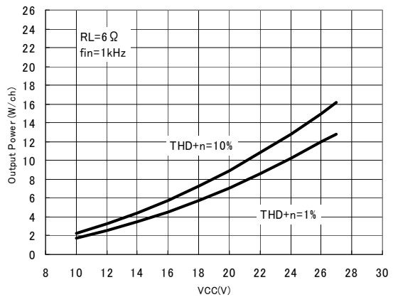
Fig.16 Power supply voltage—Output power (RL=6Ω)
