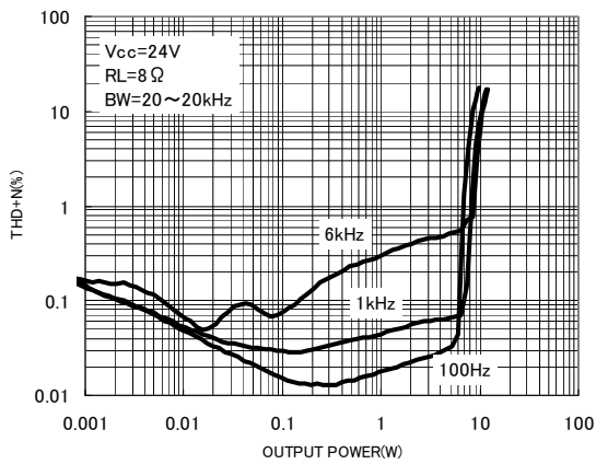
Fig.3 Output power—THD+N
