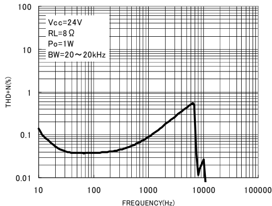
Fig.23 Frequency—THD+n
