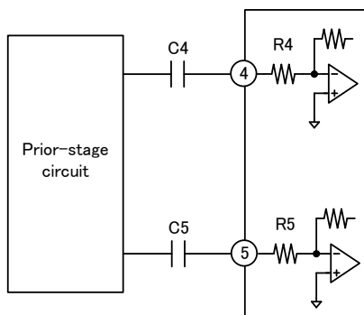
Fig. 29 Coupling capacitors of audio input pins
