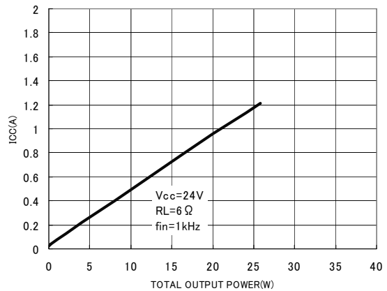
Fig.18 Total output power—Current consumption ( R_L=6\Omega )
