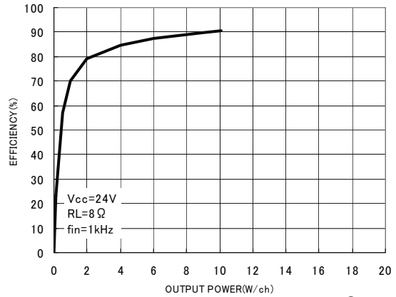
Fig.14 Output power—Efficiency ( R_L=8\Omega )
