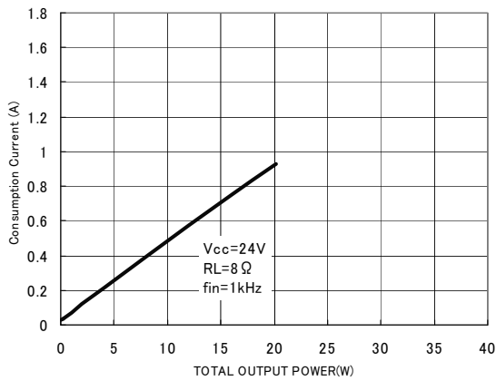
Fig.15 Total output power—Current consumption ( R_L=8\Omega )
