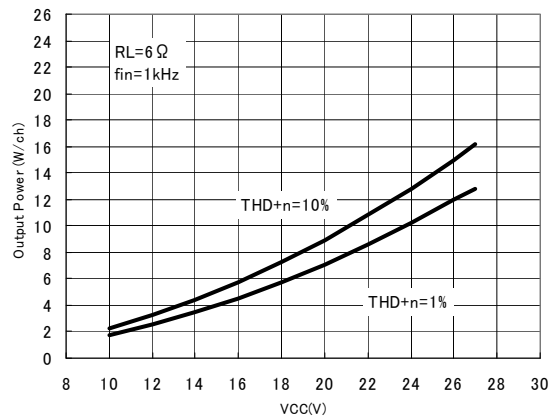
Fig.16 Power supply voltage—Output power ( R_L=6\Omega )
