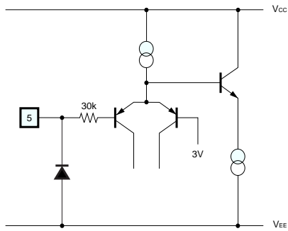
SCL (5pin)
