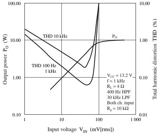
P_O , THD — V_{IN} ( R_L = 4 \Omega )
