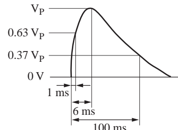
Figure 11. Surge waveform
