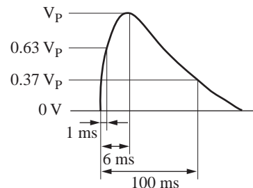
Figure 11. Surge waveform
