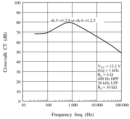
CT—freq
