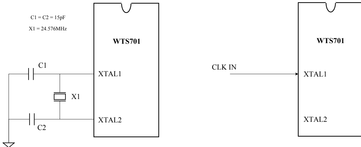
Figure 6. Clock Generation.
