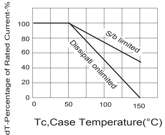
F.2 Derating Curve for All Types
