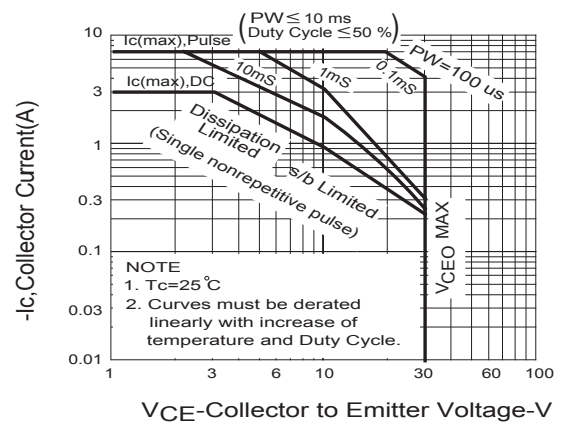
F4. Safe Operating Areas
