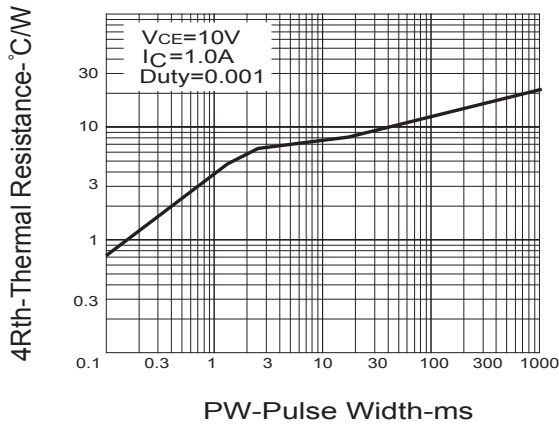
F3. Thermal Resistance VS. Pulse Width
