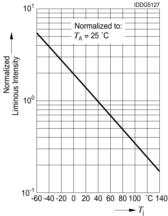
Normalized Luminous Intensity vs. Junction Temperature
