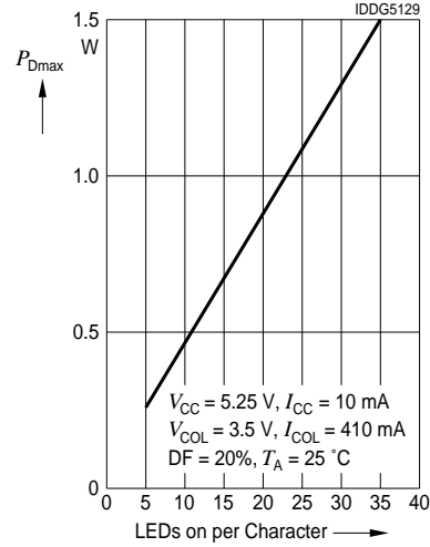
Max. Package Power Dissipation, ISD231X
