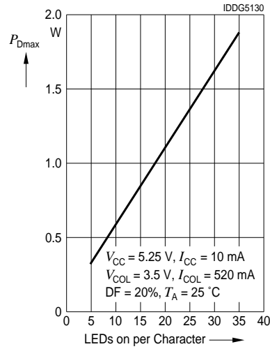
Max. Package Power Dissipation, ISD235X
