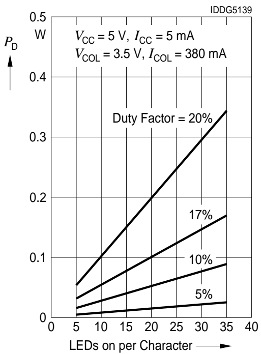
Character Power Dissipation, ISD231X
