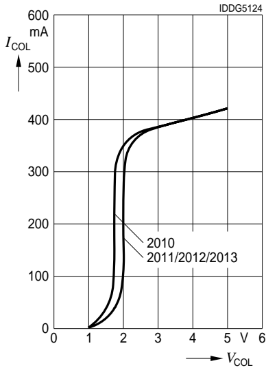
Peak Column Current vs. Column Voltage, ISD201X
