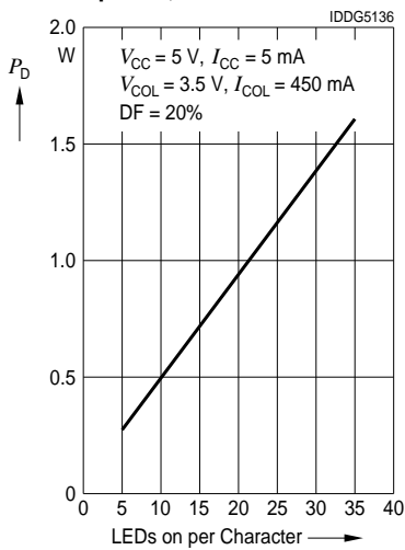
Package Power Dissipation, ISD235X
