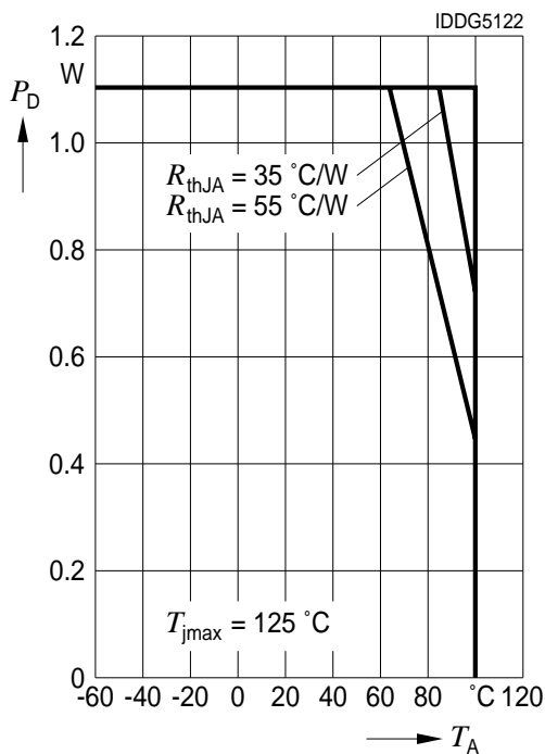
Maximum Allowable Power Dissipation vs. Temperature, ISD231X
