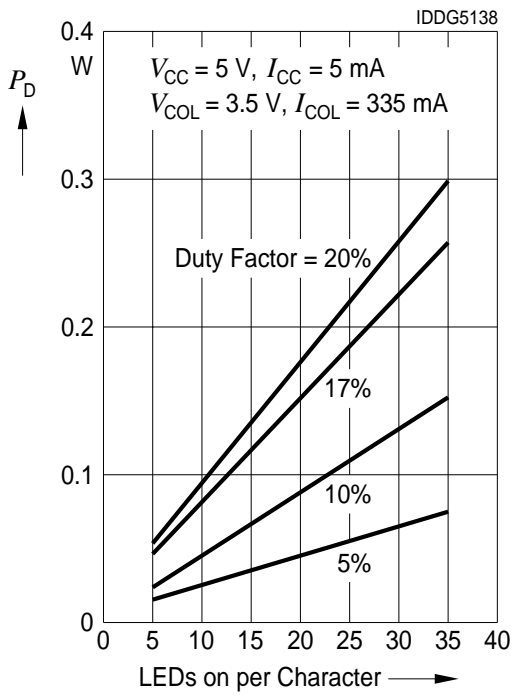
Character Power Dissipation, ISD201X
