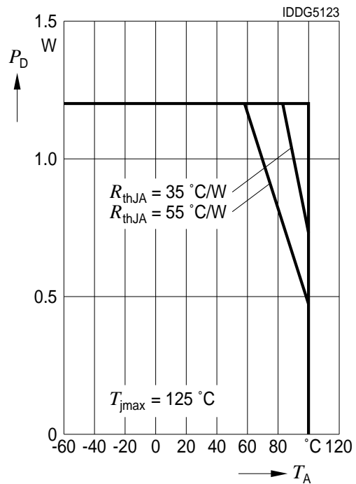
Maximum Allowable Power Dissipation vs. Temperature, ISD235X
