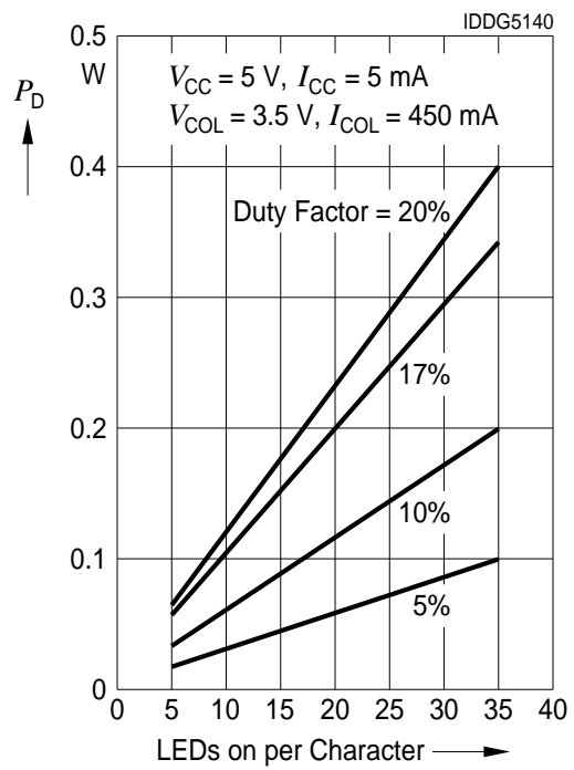
Character Power Dissipation, ISD235X
