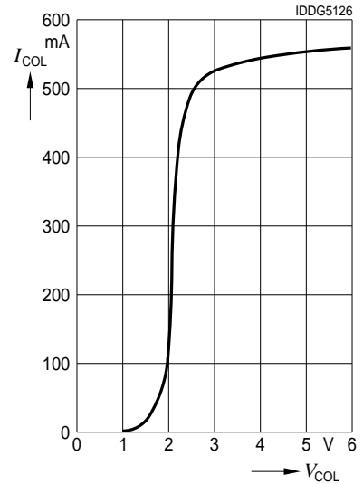
Peak Column Current vs. Column Voltage, ISD235X
