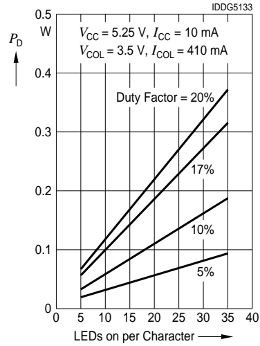
Max. Character Power Dissipation, ISD231X
