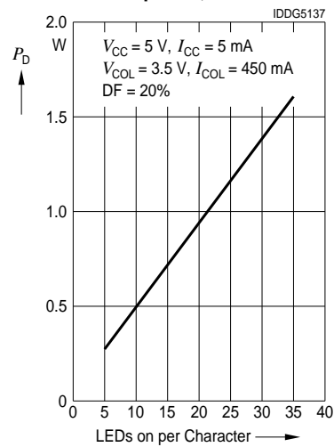
Max. Character Power Dissipation, ISD235X
