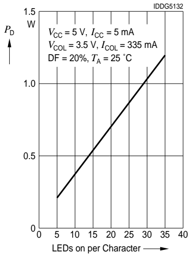
Package Power Dissipation, ISD231X
