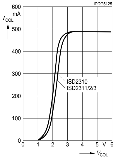
Peak Column Current vs. Column Voltage, ISD231X
